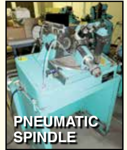
FEDERAL Mogul Mdl. 10-83-1 Drill Pointing Machine.
